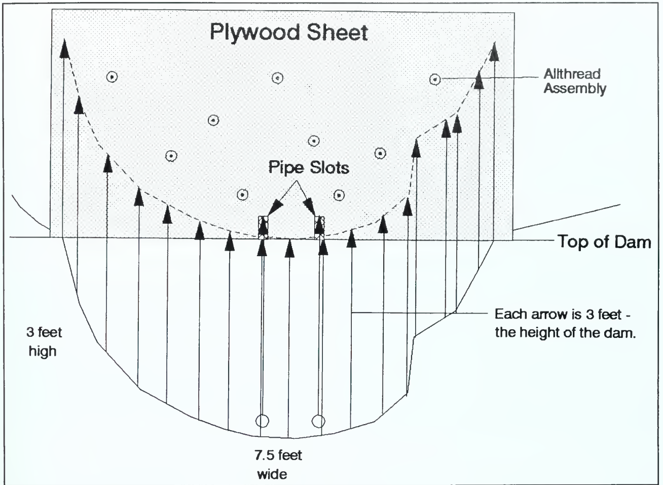
Figure 1. Dam design and materials.
